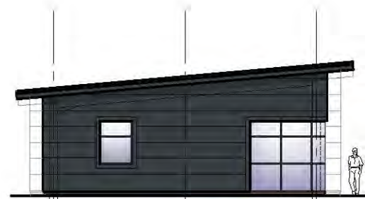
End Elevation Facing School Site (East)
